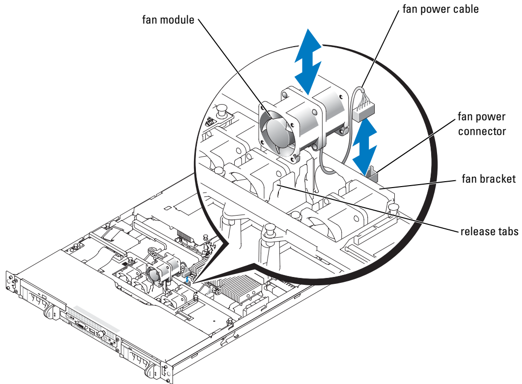
Figure 1. Removing and Installing a Fan Module
